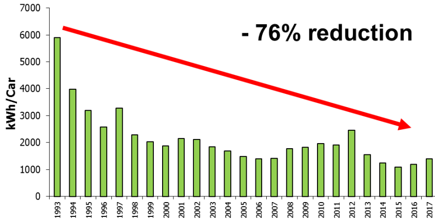
Energy usage per vehicle (kwh)
